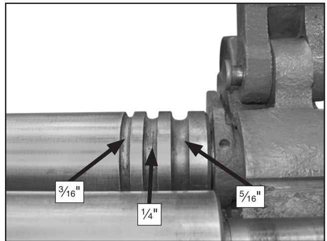
Figure 27. Wire grooves.
