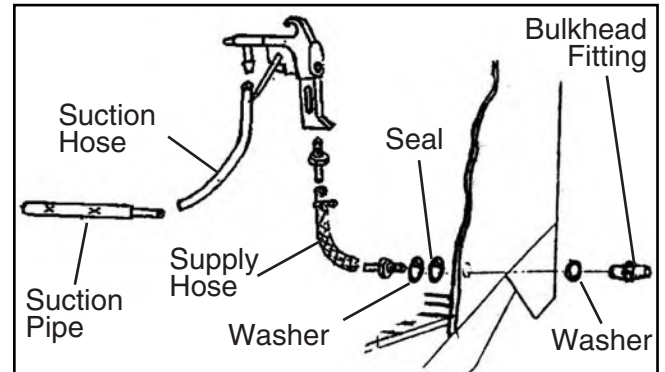
Figure 3. Blast gun assembly.
